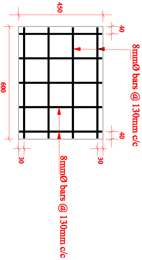
Reinforcement details in foundation
